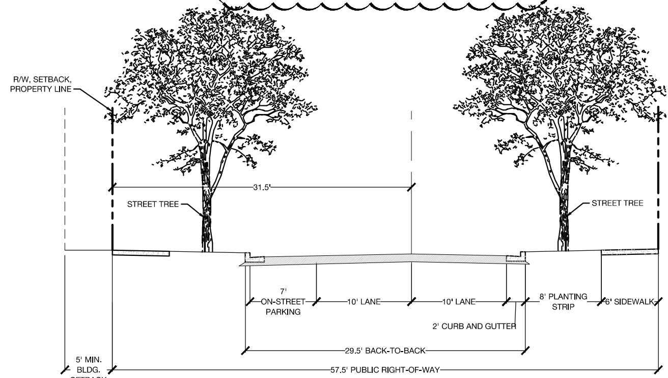
SECTION A-1 (USDG U-03A LOCAL RESIDENTIAL WIDE - MODIFIED)
