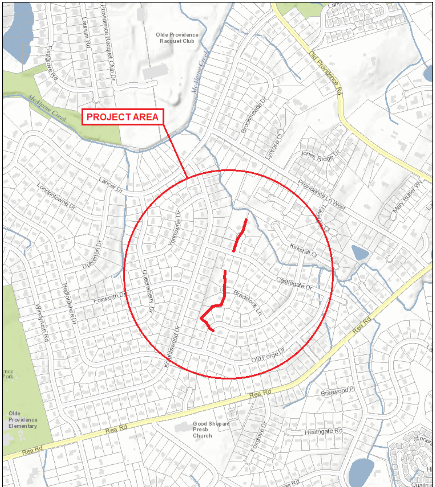
Location Map: Bradstock Lane Storm Drainage Improvement Project (Council District 7)
