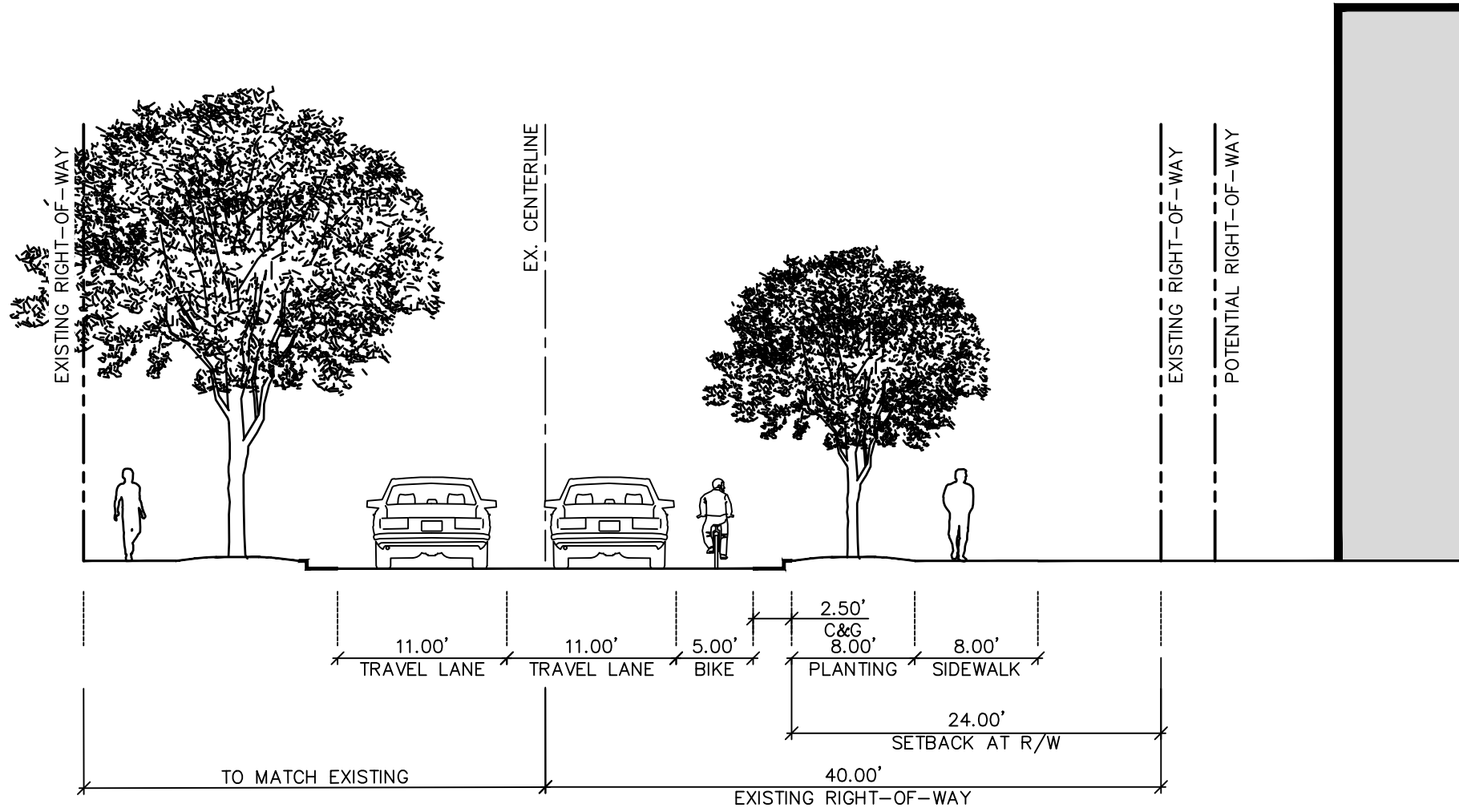
N. TRYON STREET CROSS SECTION
