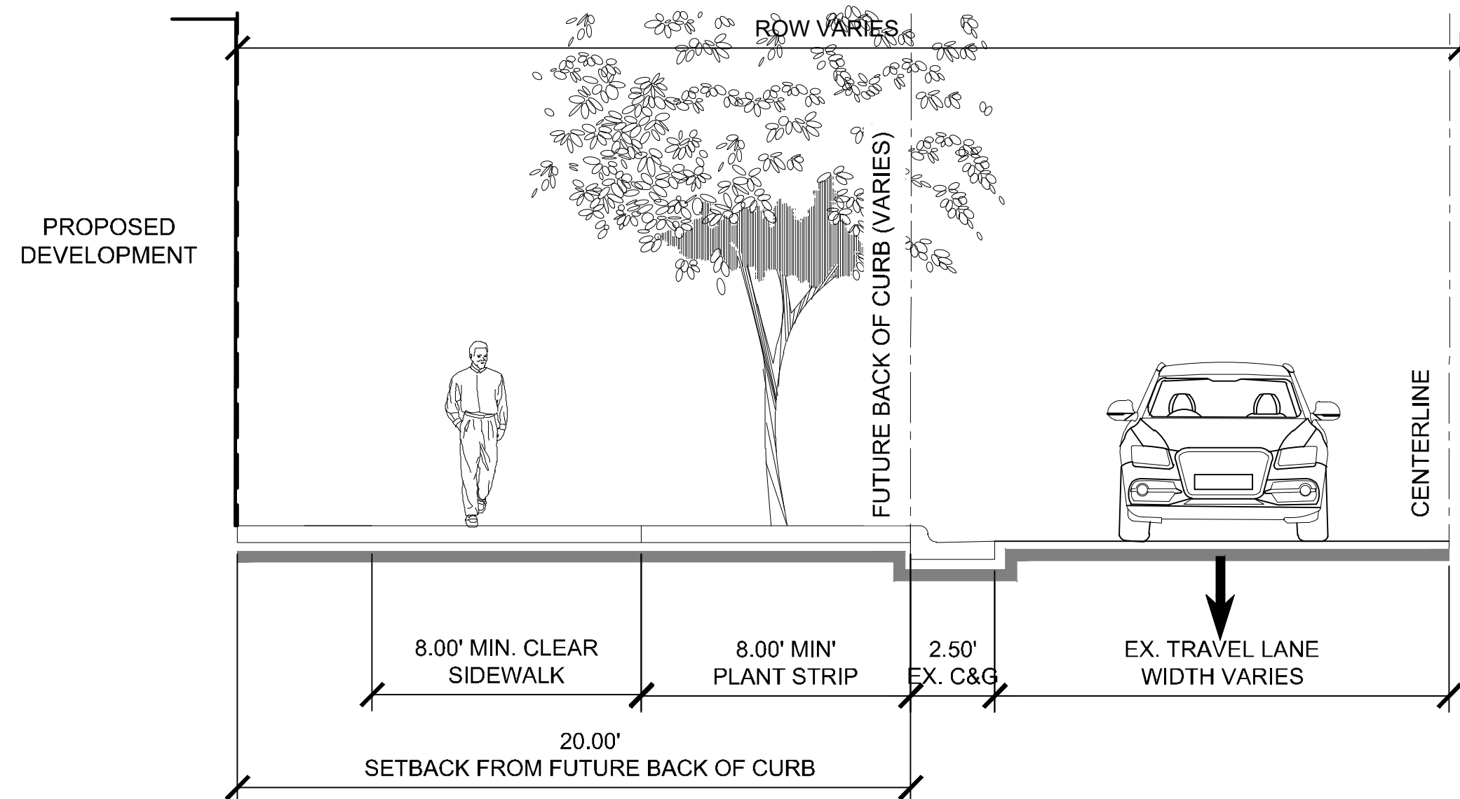
03 HAWTHORNE LN. PROPOSED CROSS SECTION
