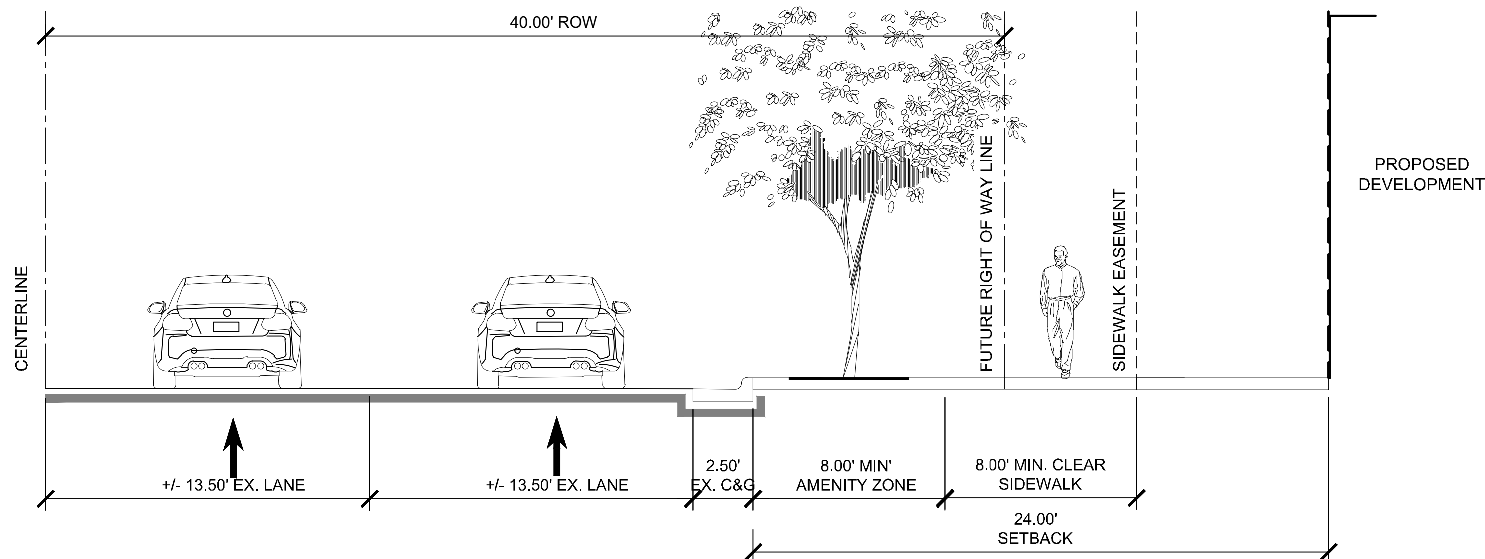
02 CENTRAL AVE. PROPOSED CROSS SECTION
