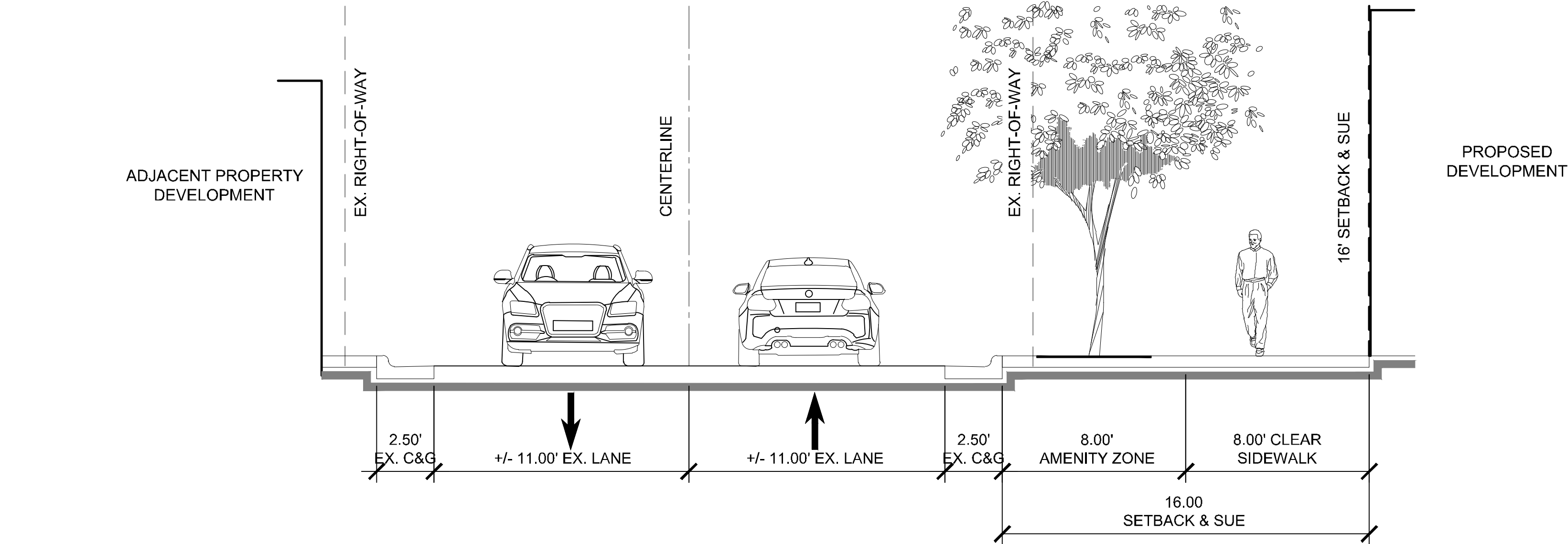
01 HEATH CT. PROPOSED CROSS SECTION
