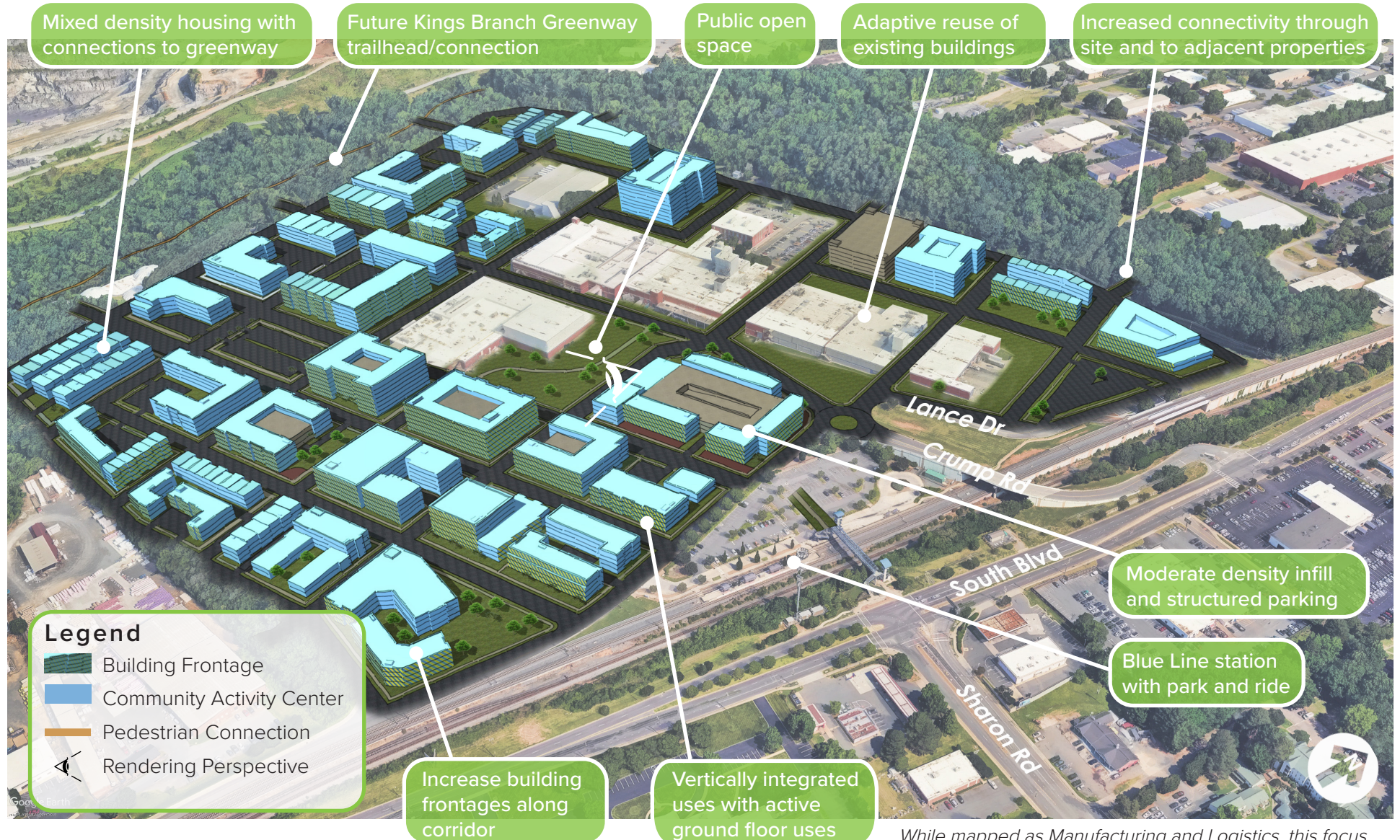
FIGURE 12: SOUTH BOULEVARD & SHARON ROAD ILLUSTRATIVE CONCEPT
