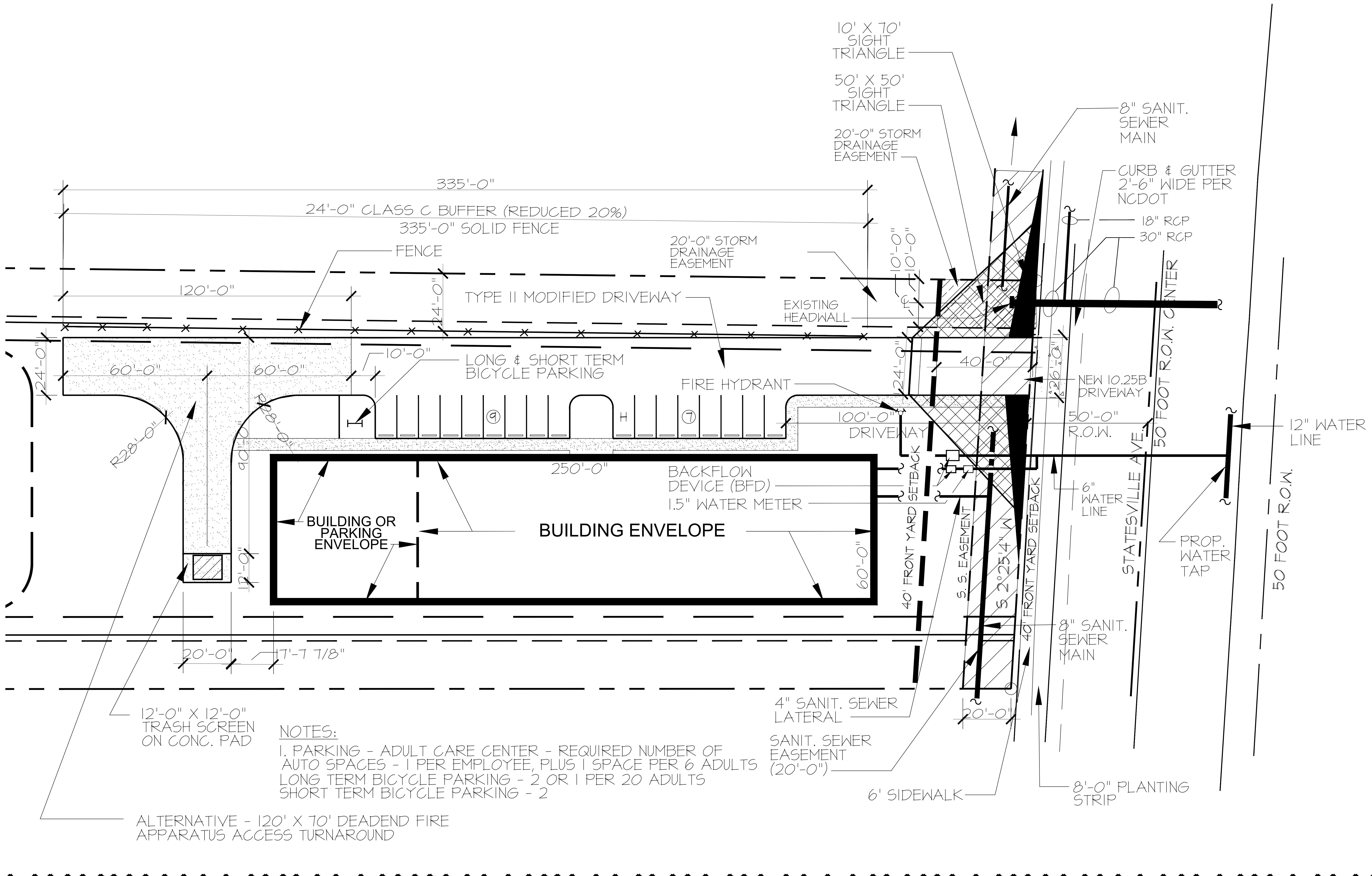
1 ENLARGED SITE PLAN 1/16" = 1'-0"
