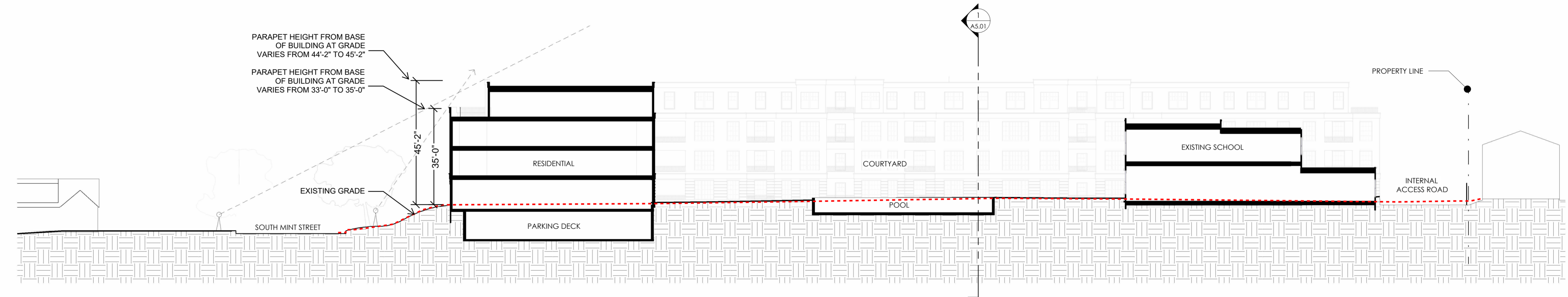
2 SITE SECTION (SOUTH MINT) SCALE: 1" = 20'-0"
