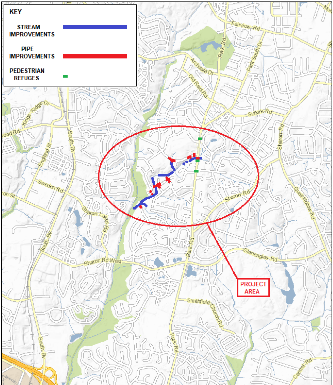
Location Map: Lilly Mill Storm Drainage Improvement and Stream Enhancement Project (Council District 6)
